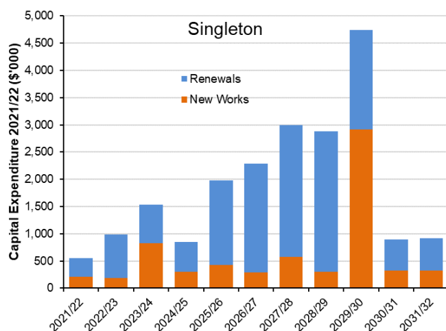
Figure 4-1: 10-year sewerage capital works program – Singleton service area
